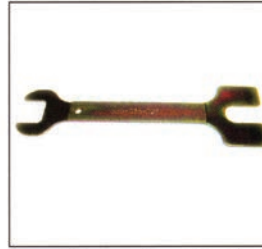
Super Charger Retaining Key Part No. 950-110 O.E. No. 529-035-949 All 4 Tec's with Super Chargers
